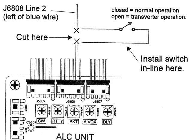
ALC Unit Modification for Transverter Operation
