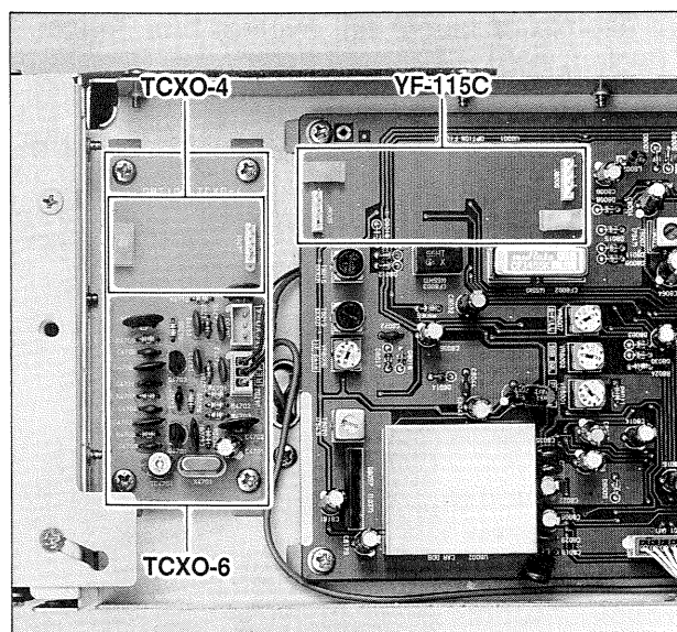
REF UNIT and SUB RX UNIT OPTION LOCATIONS
