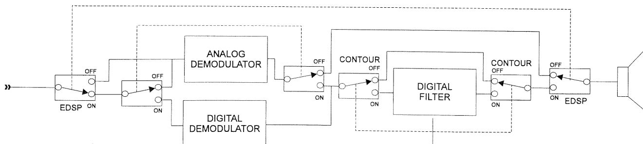
EDSP System Concept Functional Block Diagram (for illustrative purposes - actual circuit component structure may differ slightly)
