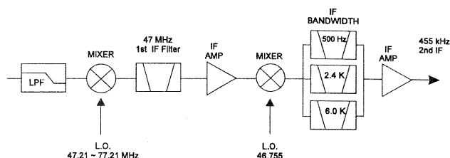
Sub Receiver IF Diagram
