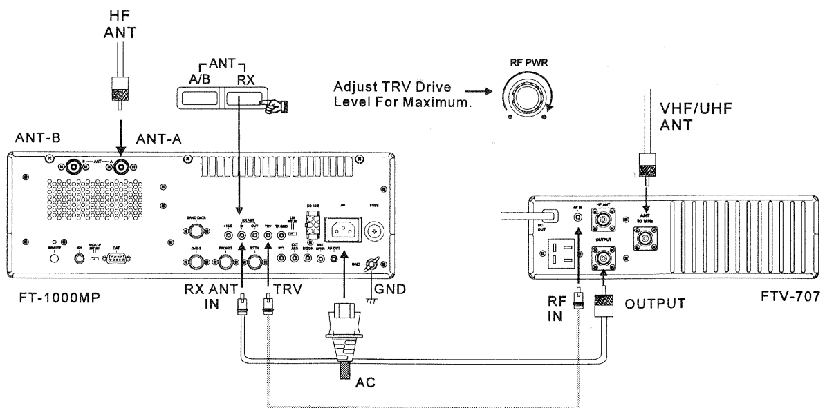
Example of Transverter Station Interconnections
