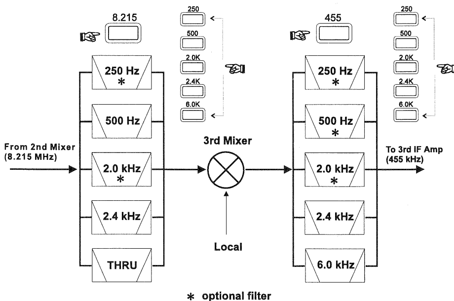
Main Receiver (VFO-A) IF Bandwidth Filter Selections
