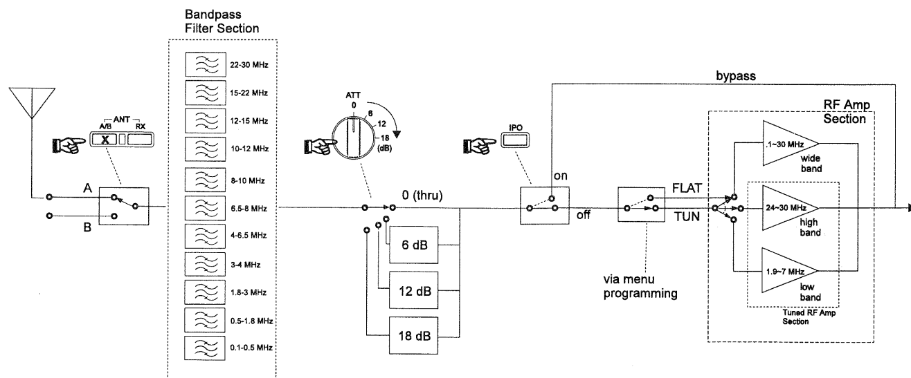
Receiver Front End Configuration (for illustrative purposes)
