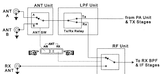
FT-1000MP Antenna Selection
