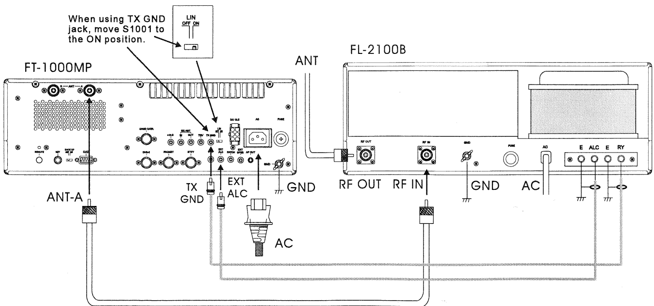
Non-QSK Linear Amplifier Interconnection
