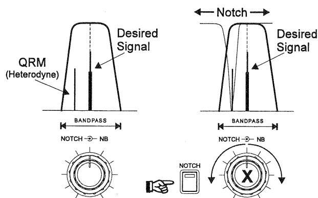
NOTCH Action
