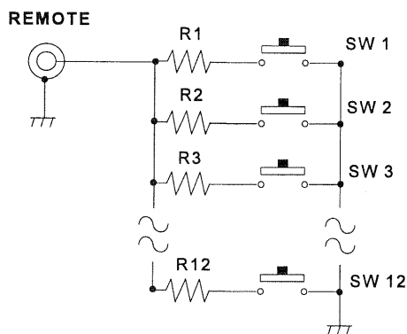
Remote Control Circuit
