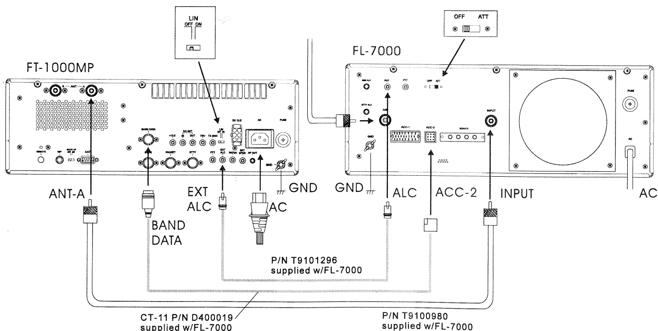
QSK Linear Amplifier Interconnections
