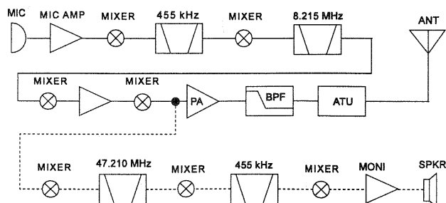
Monitor Circuit
